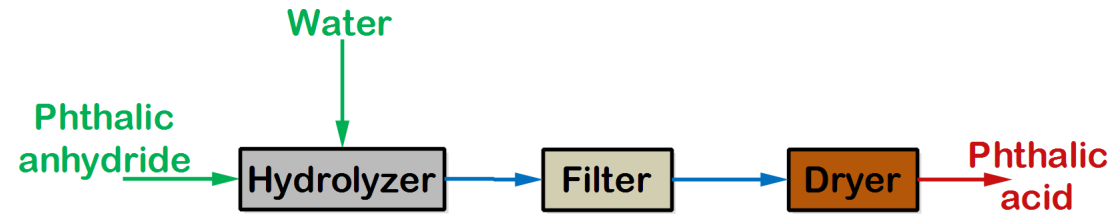
Figure: Manufacture of Phthalic acid from phthalic anhydride
